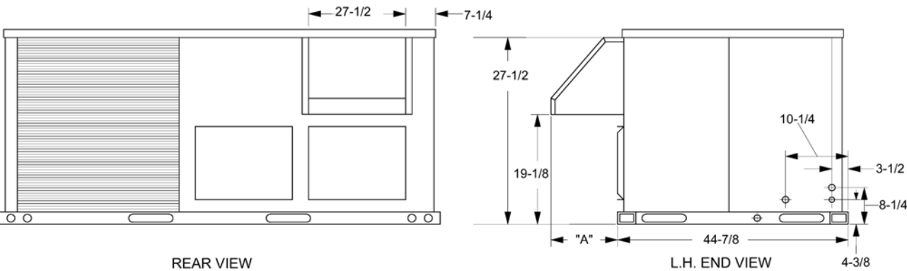
FIGURE 5 - UNIT WITH ECONOMIZER RAINHOOD
